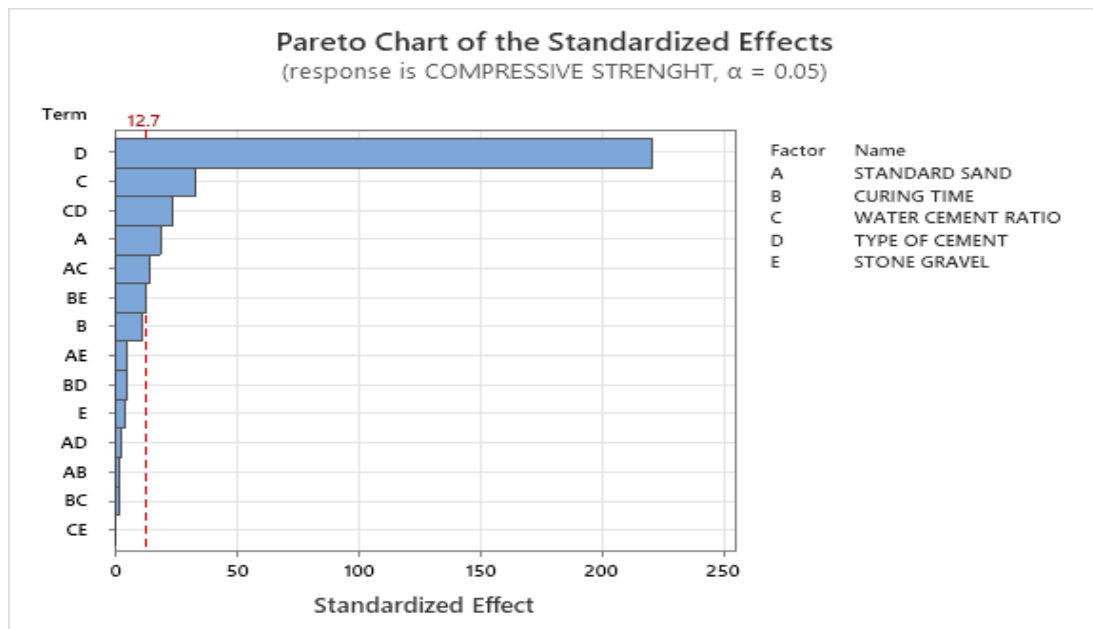
Fig. 2. Pareto chart of the standardized effects
