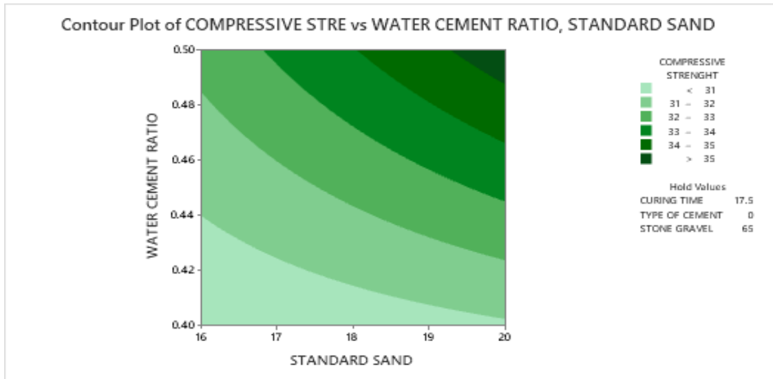
Fig. 4. Contour plot of compressive strength Vs water cement-ratio, standard sand
