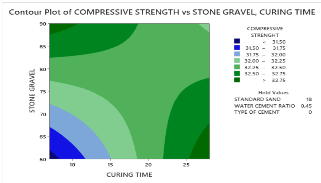
Fig. 5. Contour plot of compressive strength VS stone gravel, curing time
