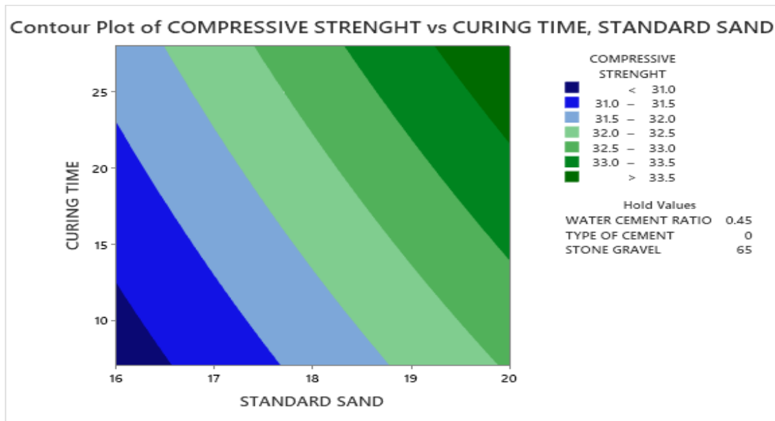
Fig. 3. Contour plot of compressive strength Vs. curing time, standard sand
